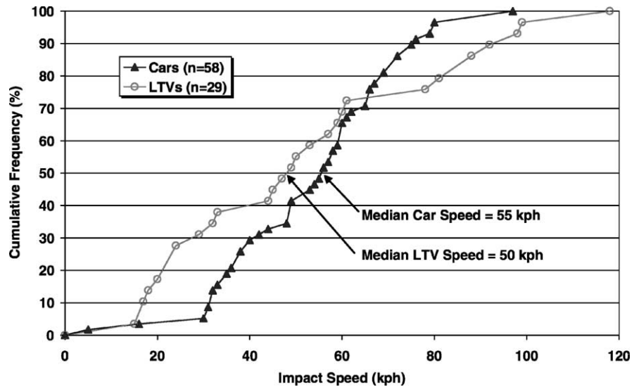
Fig. 8. Cumulative frequency of pedestrians with serious head injury AIS 3 or greater by vehicle type as a function of impact speed.
