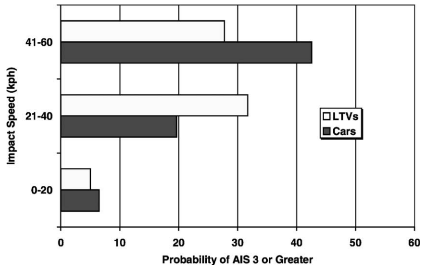
Fig. 13. Probability of serious lower extremity injury AIS 3 or greater.
