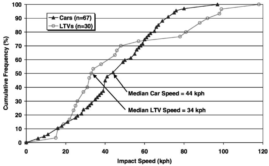
Fig. 10. Cumulative frequency of pedestrians with serious lower extremity injury AIS 3 or greater by vehicle type as a function of impact speed.
