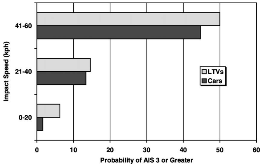
Fig. 11. Probability of serious head injury AIS 3 or greater.
