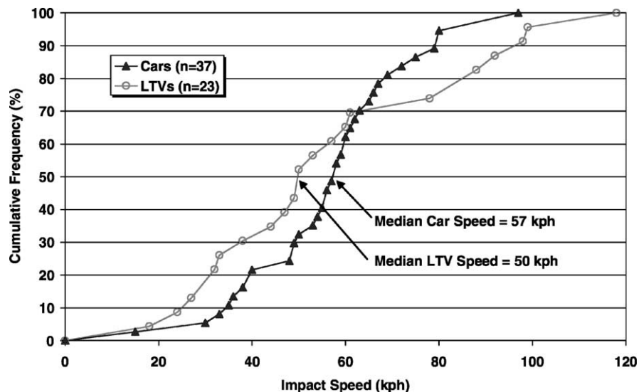
Fig. 9. Cumulative frequency of pedestrians with serious chest injury AIS 3 or greater by vehicle type as a function of impact speed.
